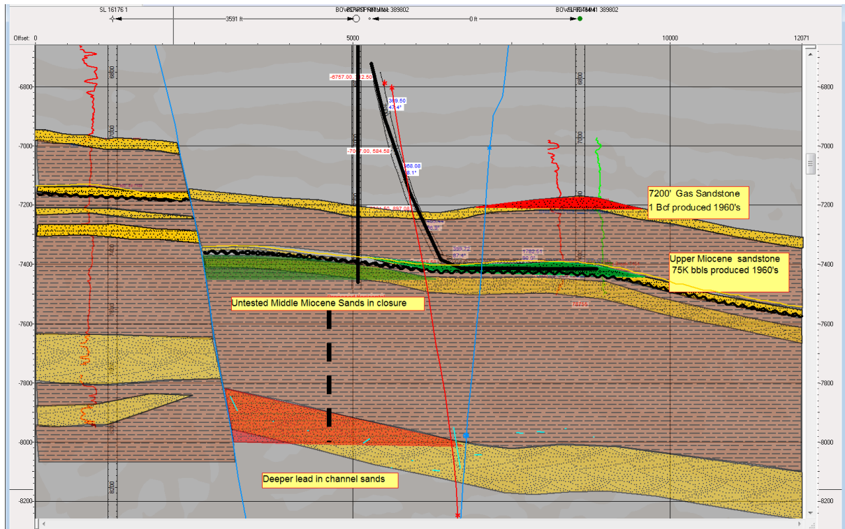
Figure 1 - Cross Section through Bowsprit Project illustrating flowed and prospective targets at depths of 7,200 ft to 8,000ft.
