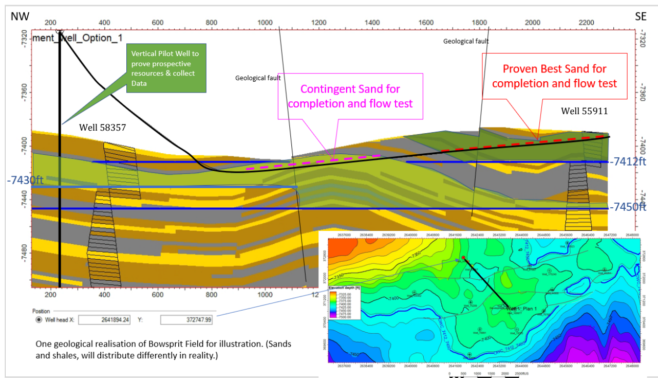
Figure 1 - Vertical Pilot hole and Horizontal Well Path
