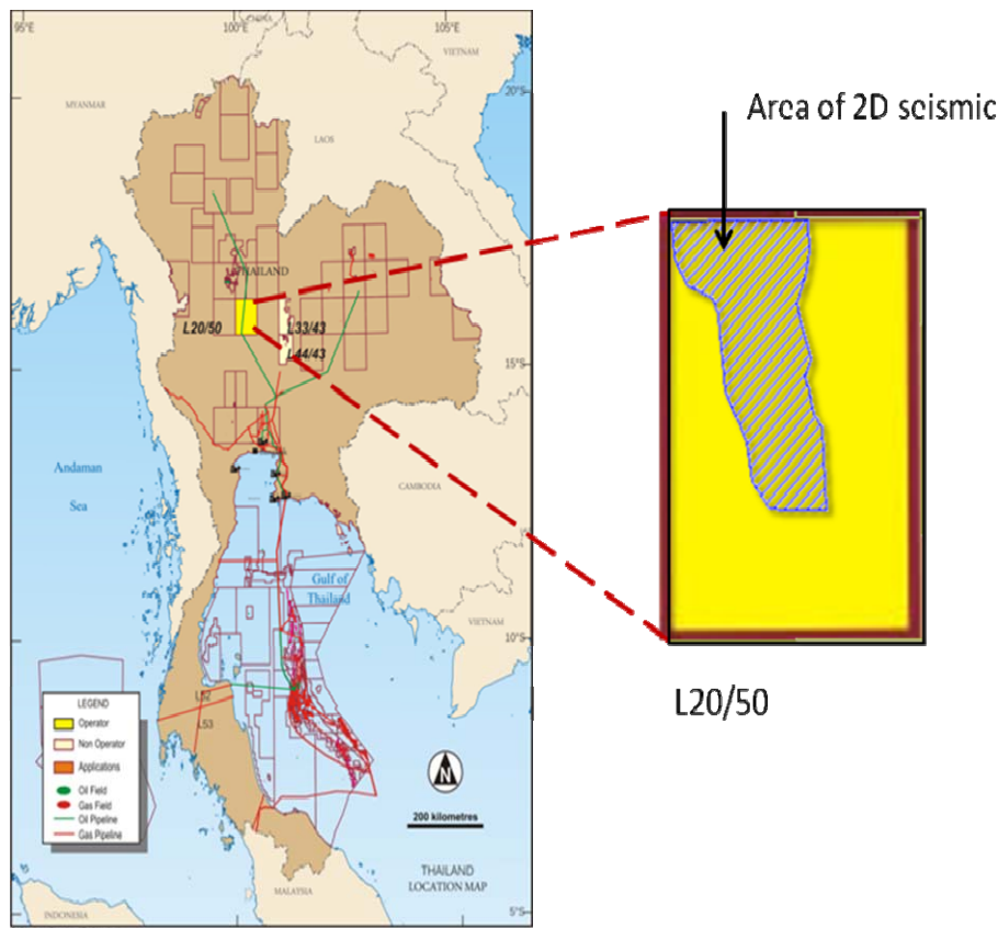
Location of L20/50, Thailand, showing outline of seismic survey
