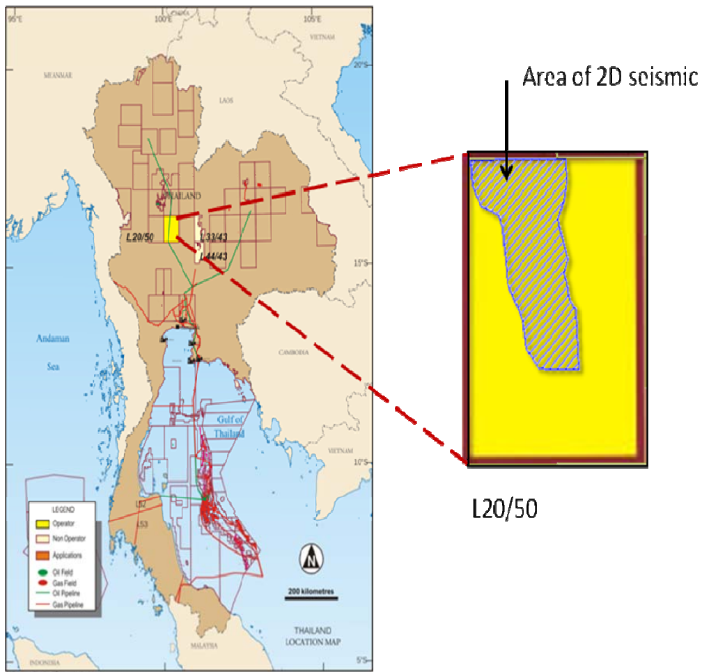
Location of L20/50, Thailand showing seismic survey
